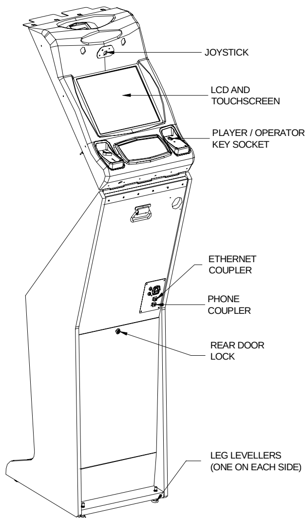
FIGURE 29 - REAR VIEW OF THE FUSION WITH BEZEL OPEN
