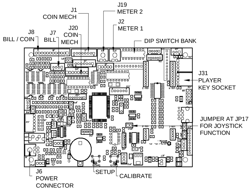
FIGURE 32 - I/O BOARD DRAWING
